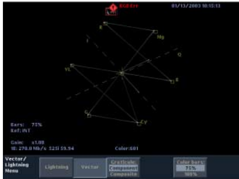
Figure 2-33: Vector display with component graticule selected and with compass rose turned off
