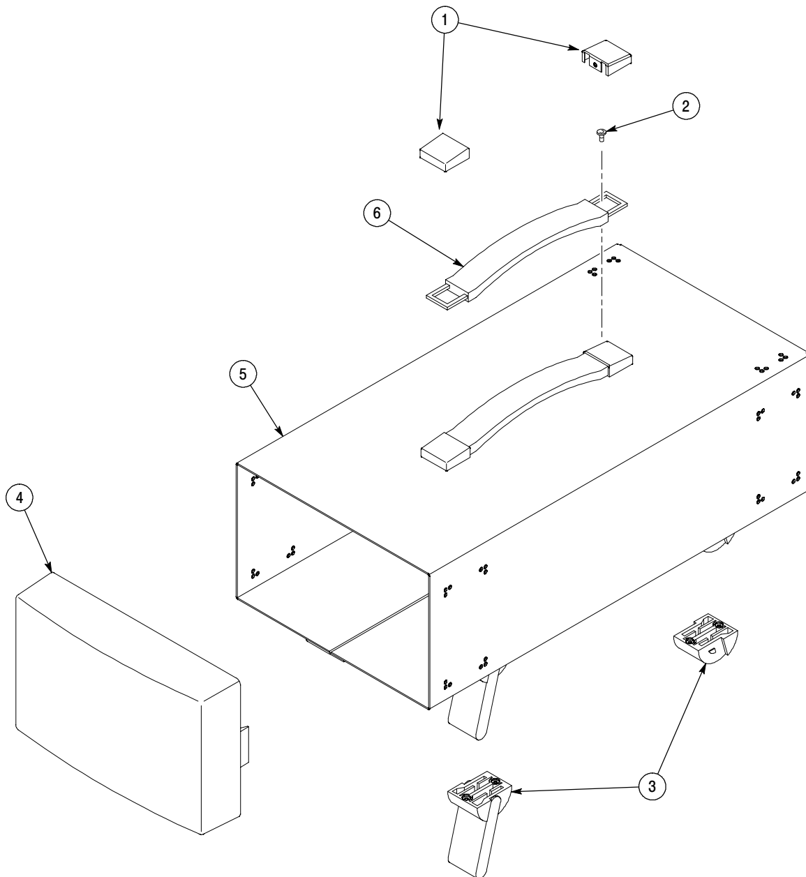
Figure 3- 5: WFM7F02 replaceable parts
