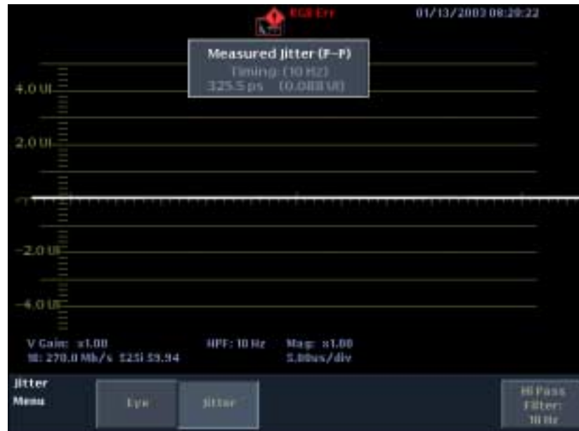
Figure 2- 15: Jitter measurement display
