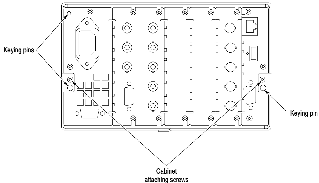
Figure 3-8: WFM7F03 rear-panel attaching screws
