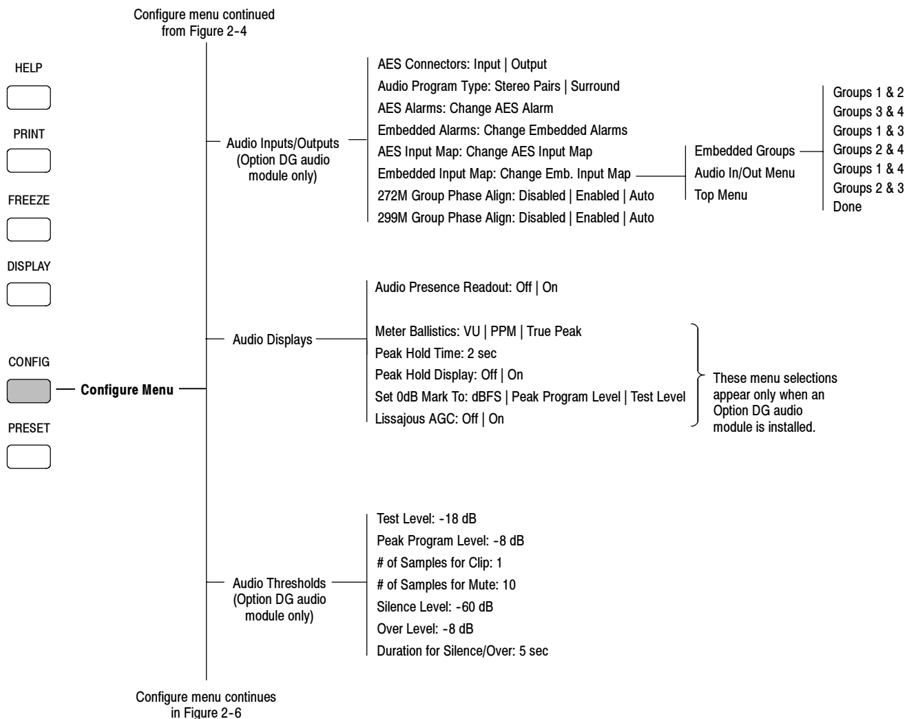
Figure 2- 5: Configuration menu diagram - part 3
