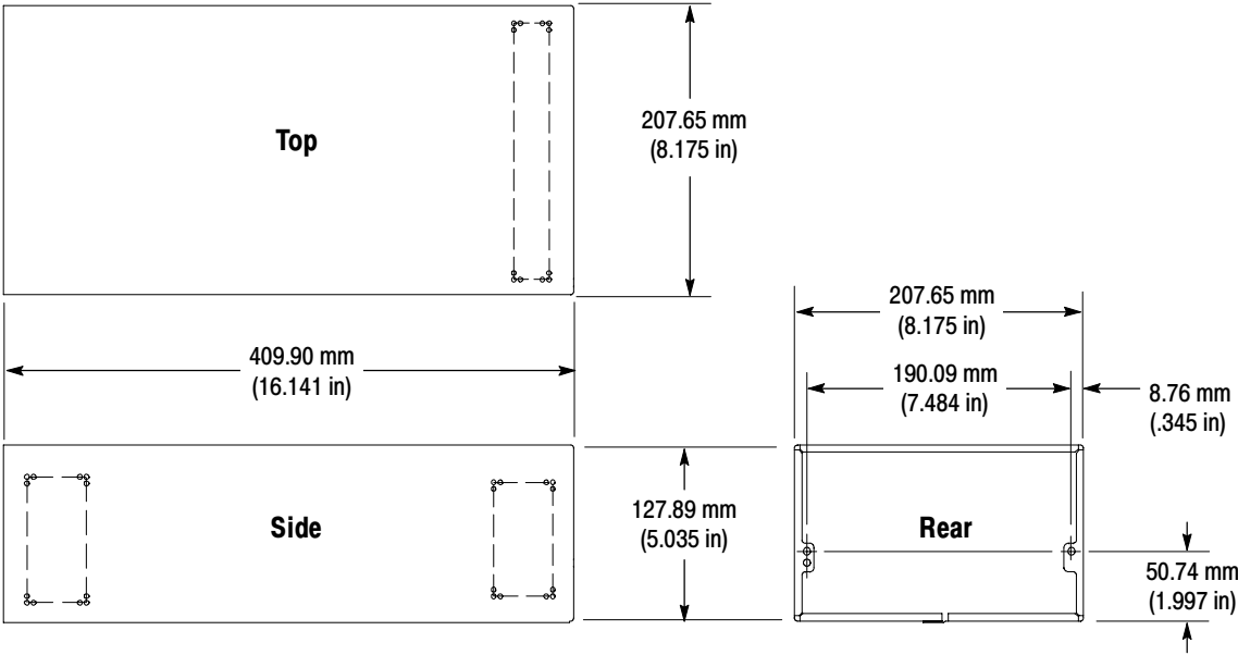
Figure 3-3: WFM7F02 cabinet dimensions
