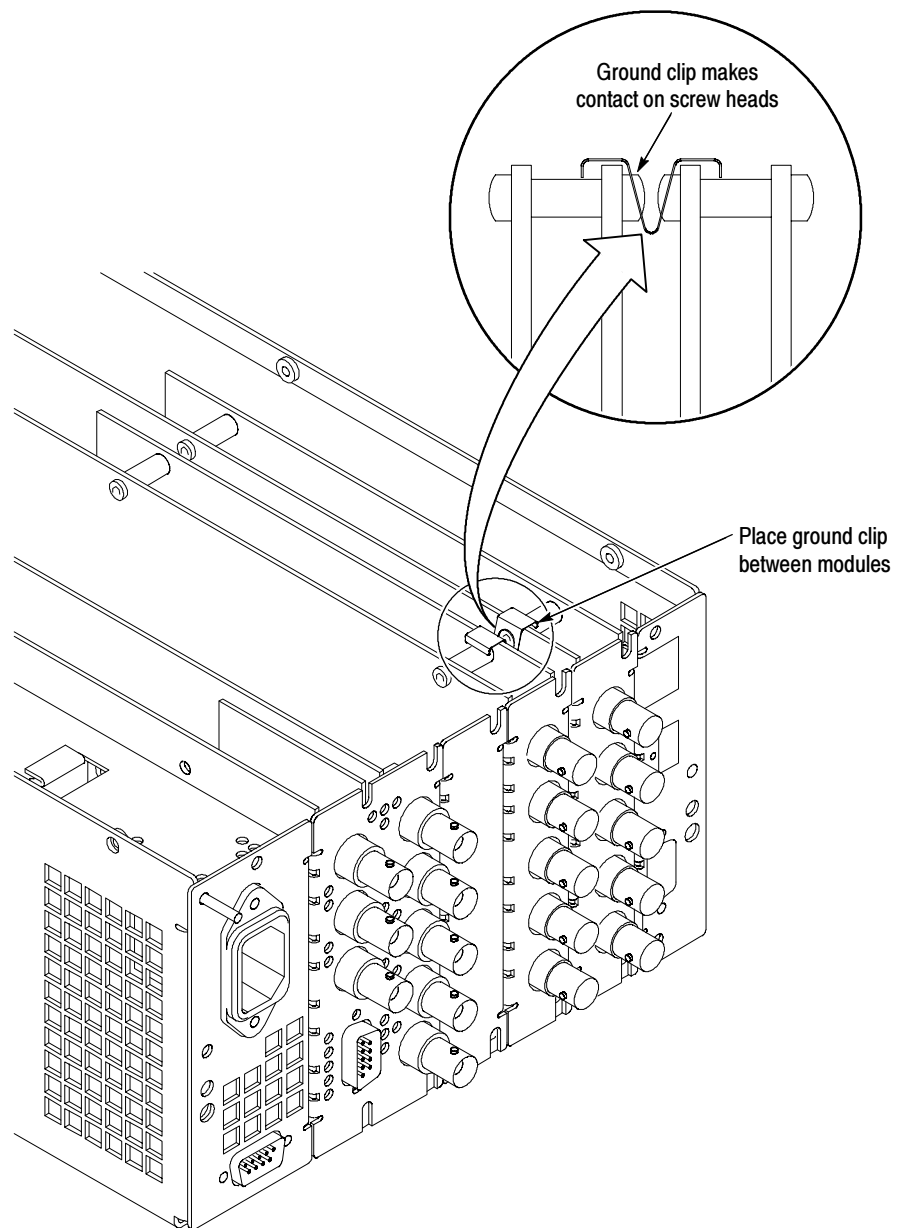
Figure 3-20: Installing the grounding clip between two video modules
