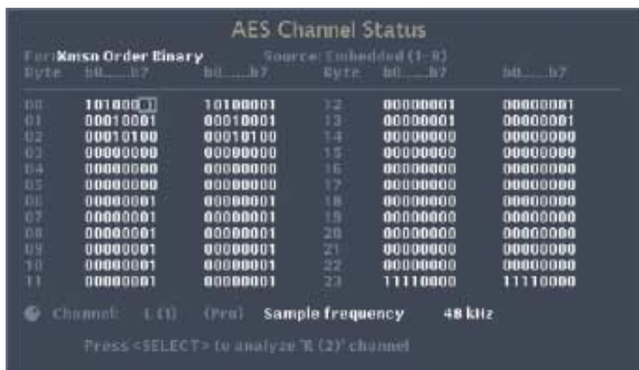
Figure 2-46: Channel Status display in XMSN Order Binary format
