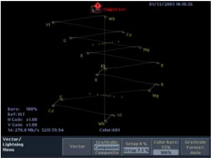
Figure 2- 32: Lightning display
