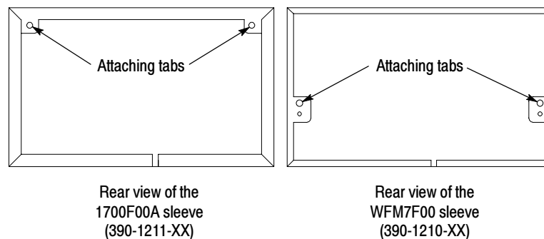
Figure 3-14: Rear view of the WFM7F05 sleeves, showing the locations of the attaching tabs and screws
