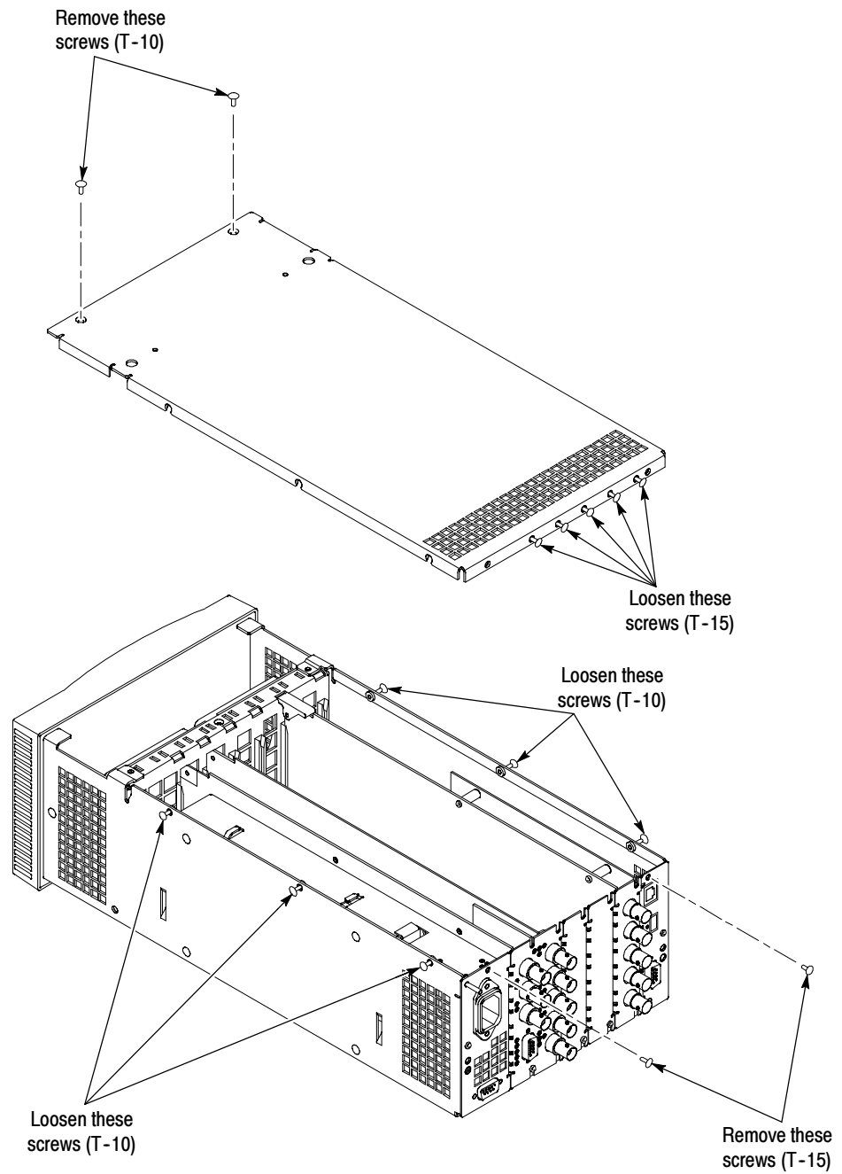
Figure 3- 18: WFM700 chassis, showing screws to loosen and remove
