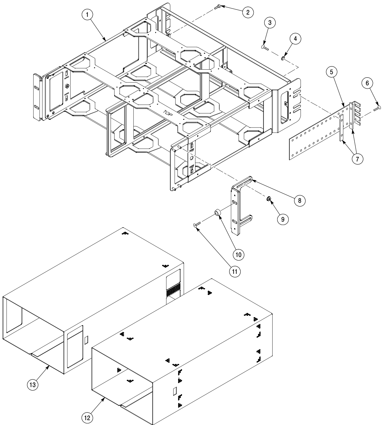
Figure 3- 16: WFM7F05 rack adapter replaceable parts
