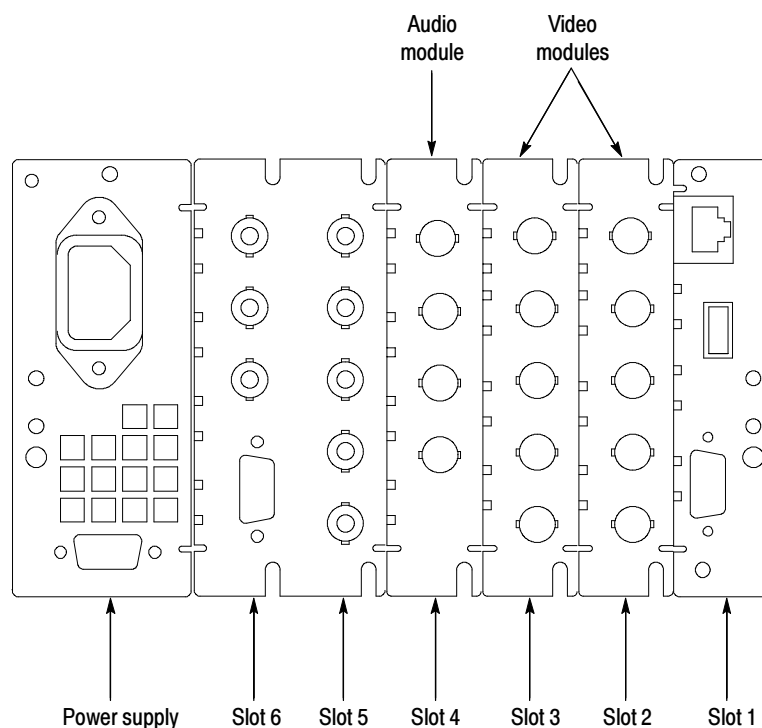
Figure 3-17: WFM700 rear panel slot numbers (two video modules and one audio module installed)
