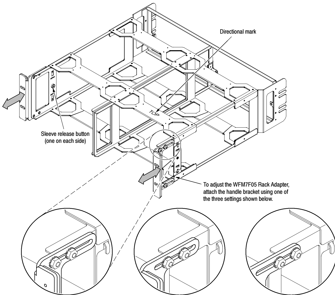
Figure 3-13: Adjusting the position of the WFM7F05 rack adapter handles
