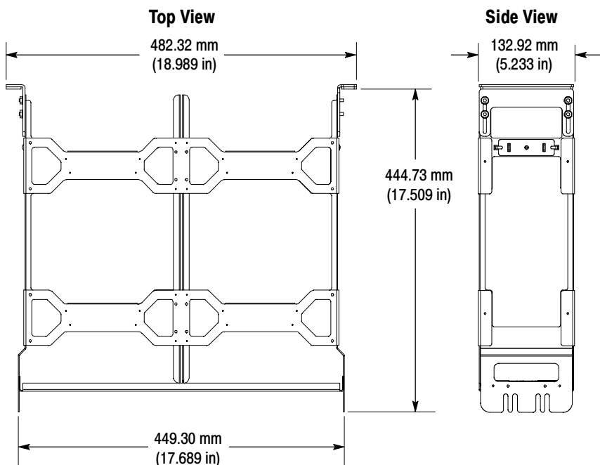
Figure 3- 10: WFM7F05 rack adapter dimensions
