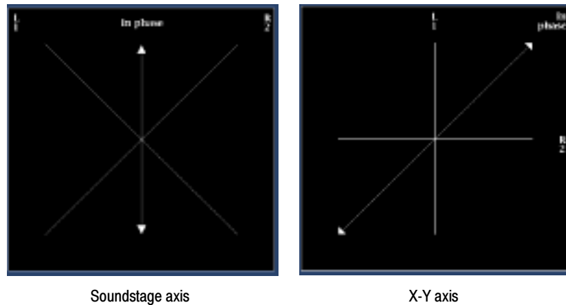
Figure 2-43: Axis styles used by the Lissajous display
