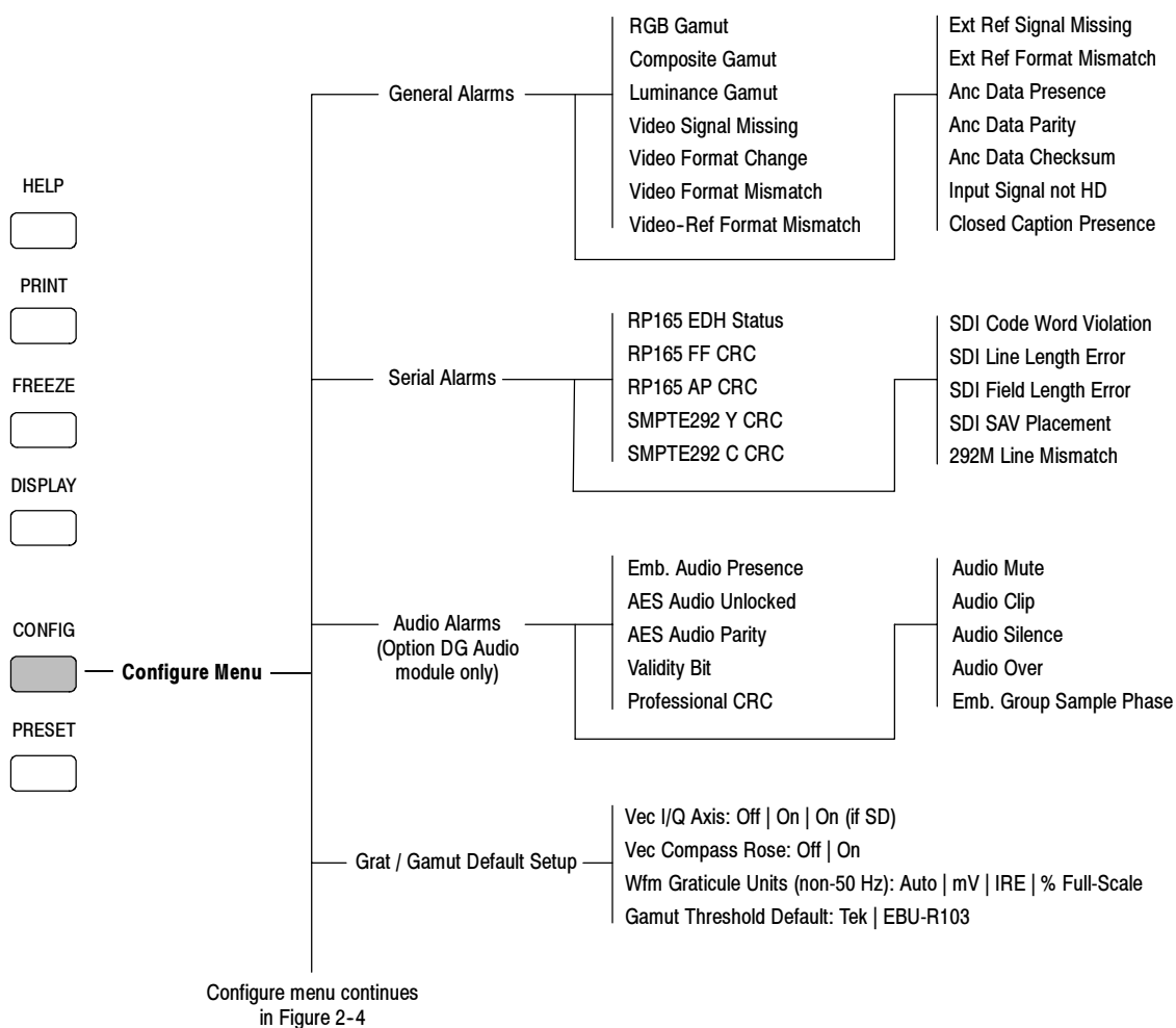
Figure 2-3: Configuration menu diagram - part 1
