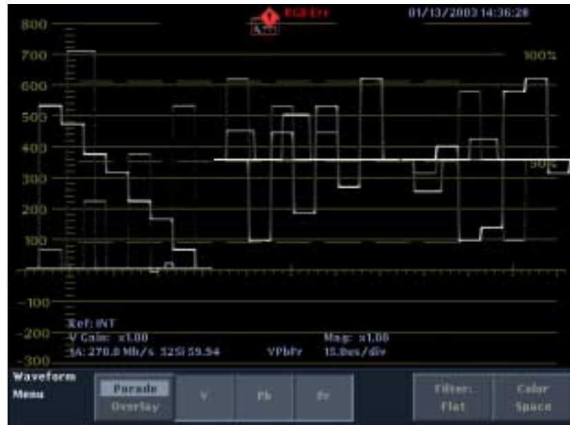
Figure 2-36: Waveform mode showing a YPbPr Parade display
