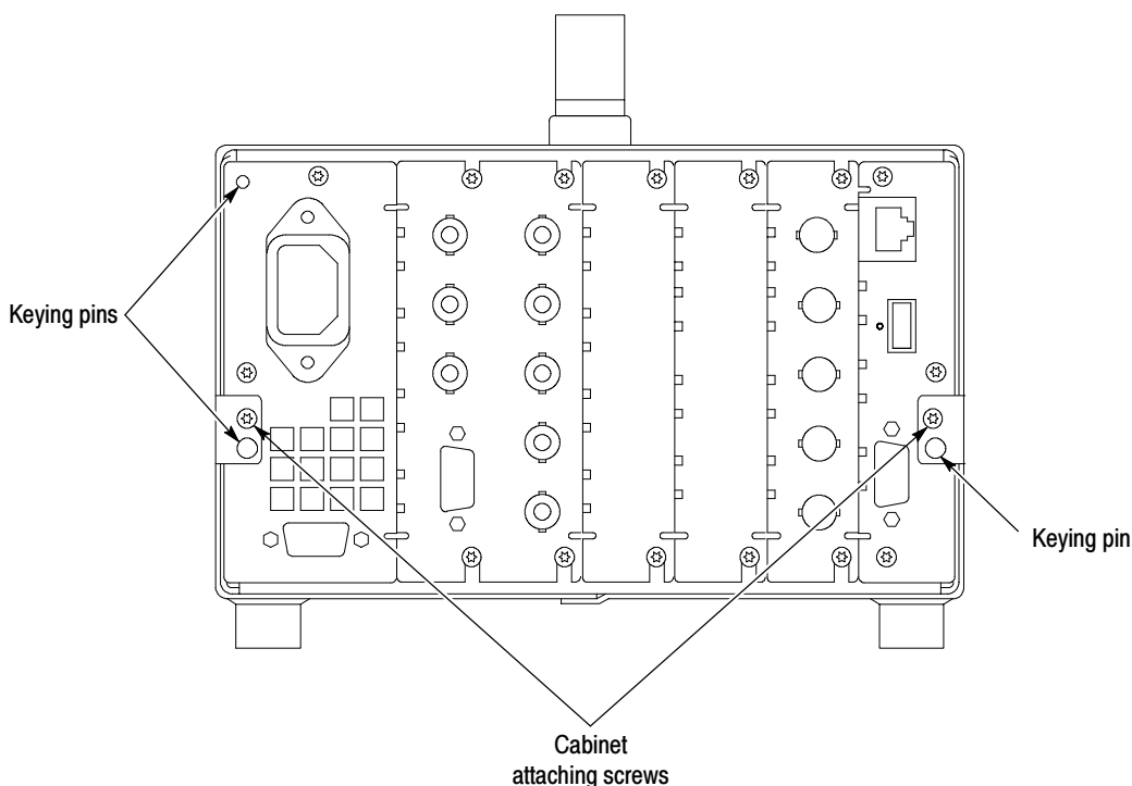
Figure 3- 4: WFM7F02 rear-panel attaching screws
