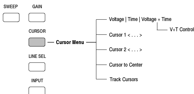
Figure 2-10: Cursor menu diagram
