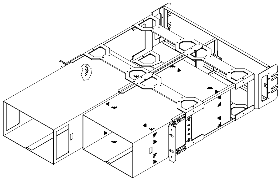
Figure 3-9: WFM7F05 rack adapter
