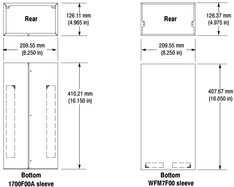
Figure 3- 11: WFM7F05 sleeve dimensions
