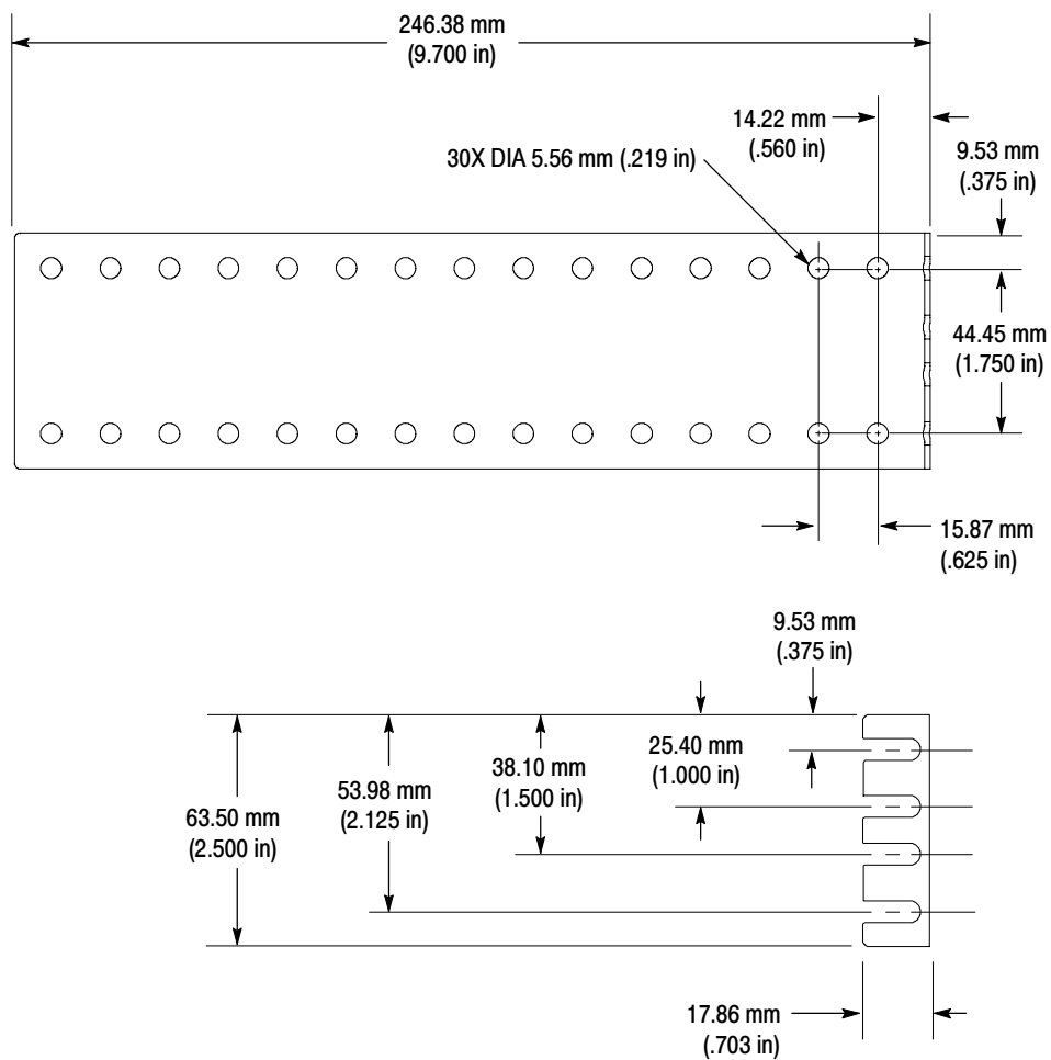
Figure 3- 12: Rear bracket guide dimensions
