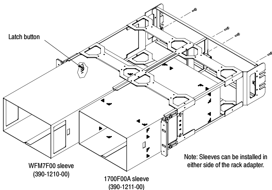
Figure 3- 15: Installing the sleeves into the WFM7F05 rack adapter
