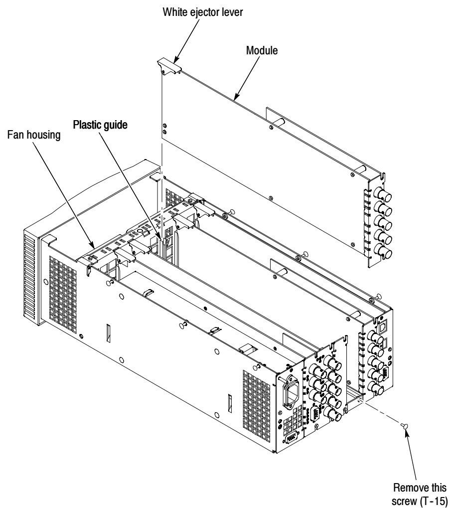
Figure 3-19: Inserting the module into the chassis
