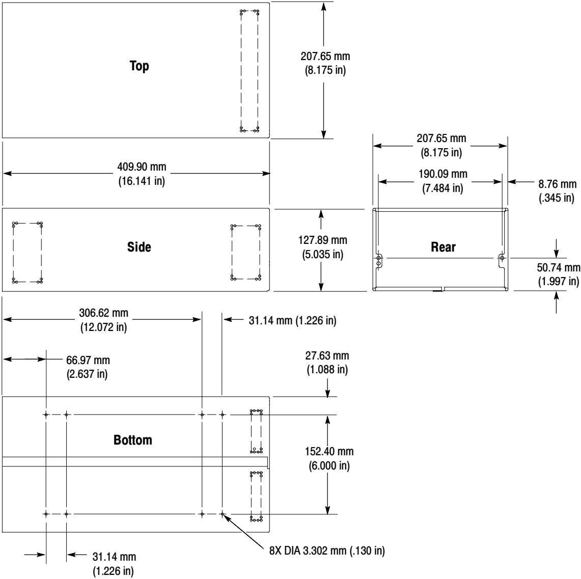
Figure 3-7: WFM7F03 cabinet dimensions
